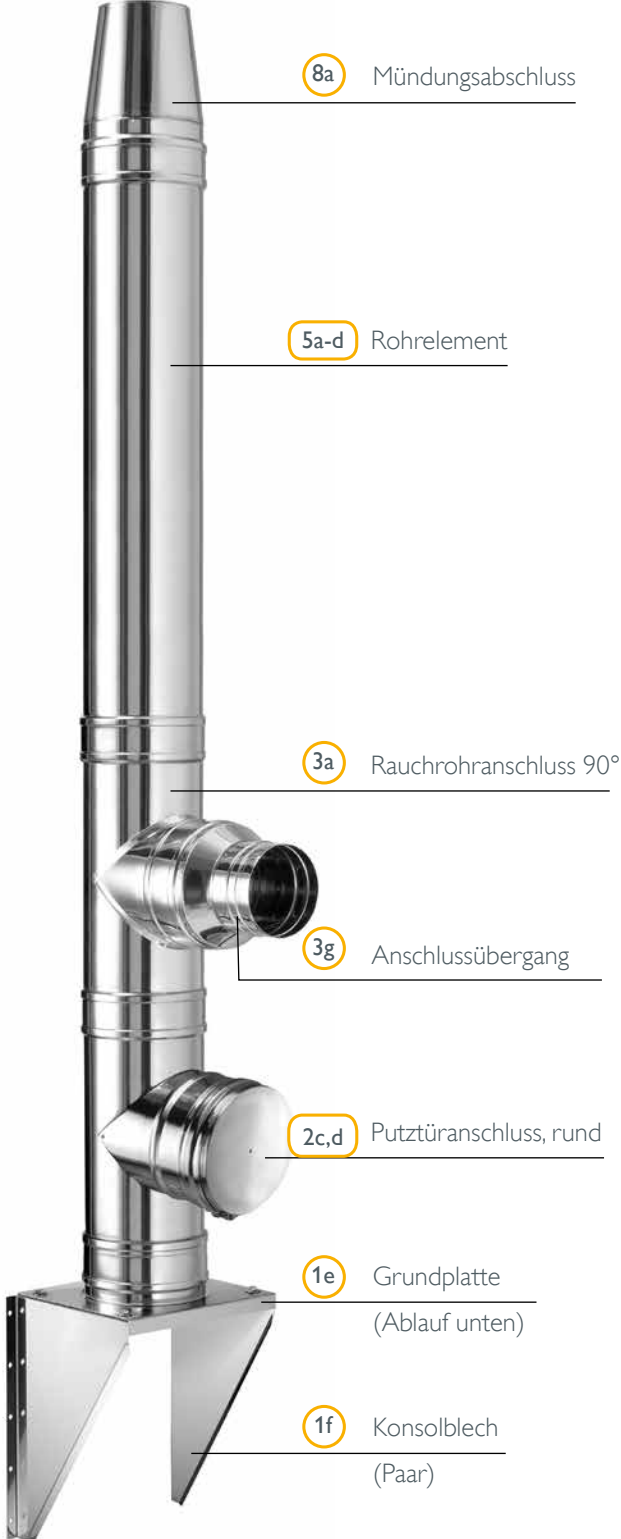
Wandmontage
