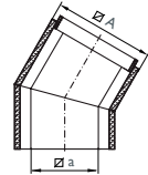
LB90 – Bogen 30°
