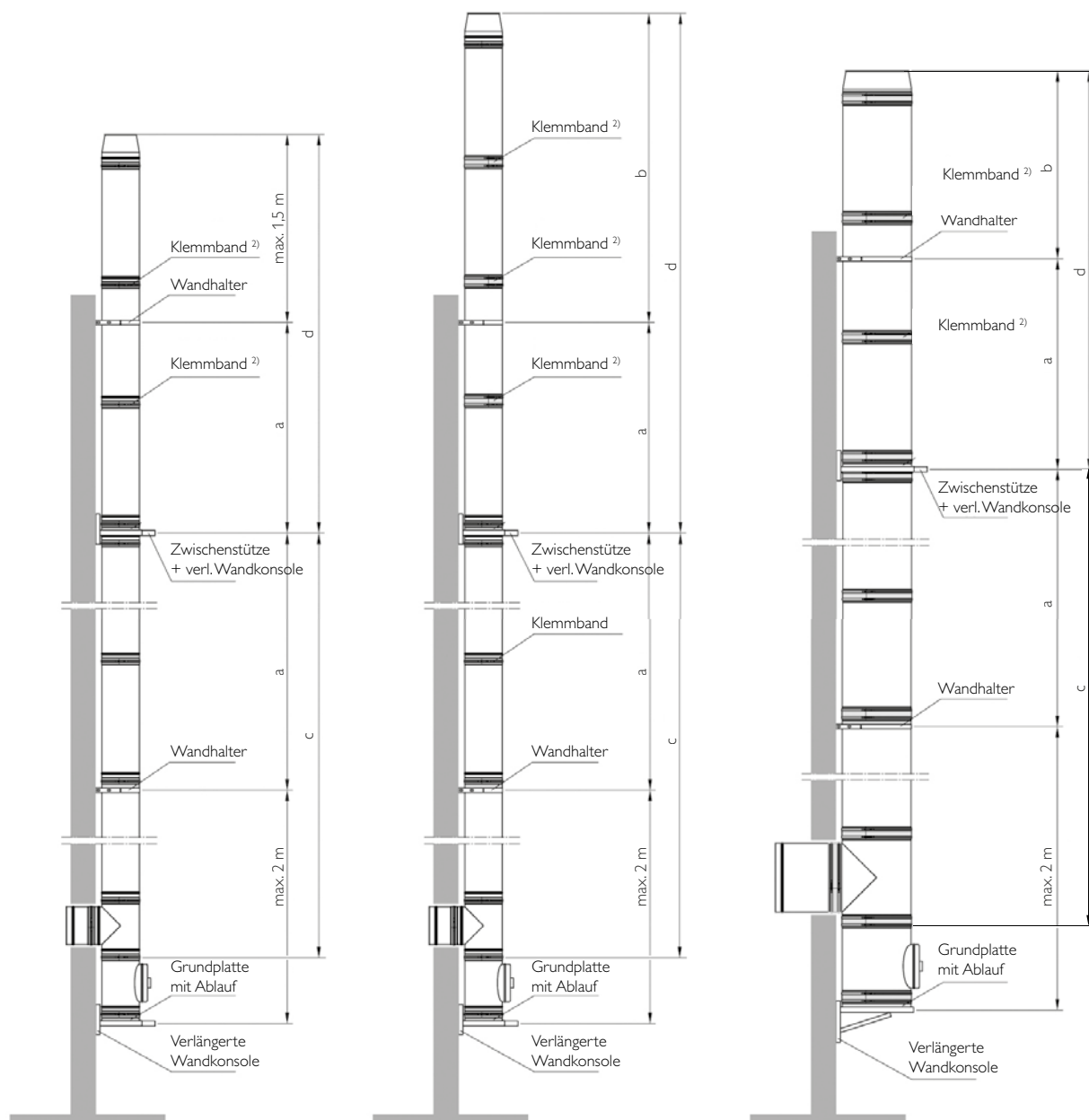
ICS Ø 80-700
