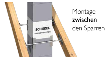
Kaminhalter Standard
