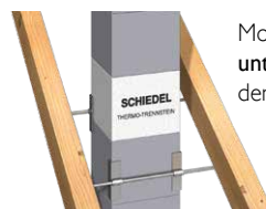
Kaminhalter Standard
