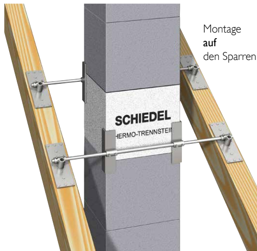
Kaminhalter Standard
