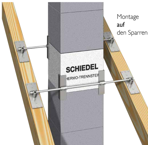
Kaminhalter Standard
