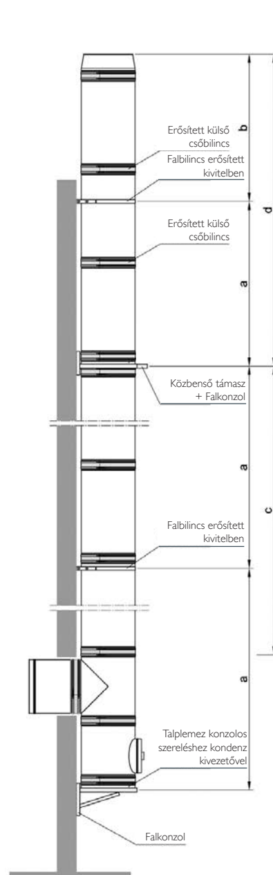
ICS Ø350-700
